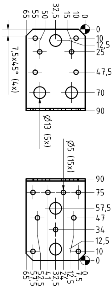
Figure A. 3 Dimensions of Angle Bracket 1132
