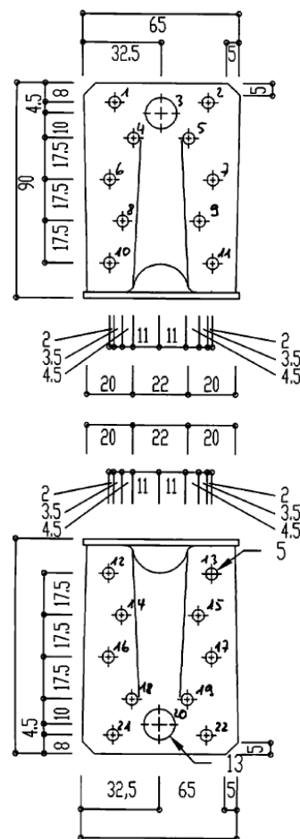
Figure A. 4 Dimensions of Angle Bracket 1112
