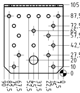
Figure A. 5 Dimensions of Angle Bracket 1133
