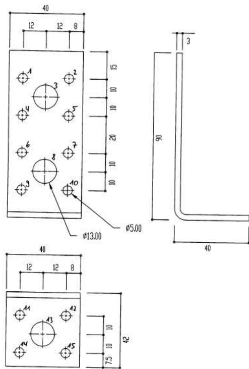
Figure A. 4 Dimensions of Angle Bracket 1136
