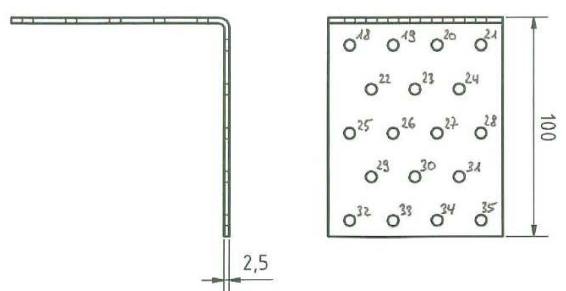
Figure A. 24 Dimensions of Angle Bracket 1232
