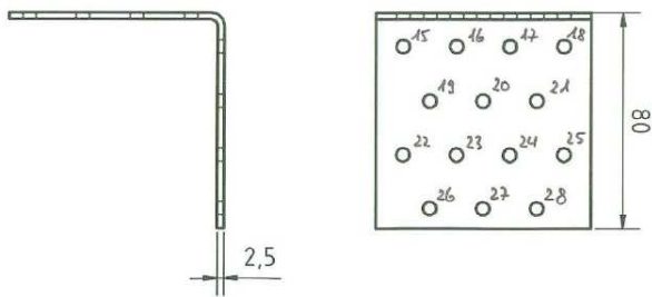
Figure A. 23 Dimensions of Angle Bracket 1231
