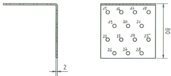
Figure A. 14 Dimensions of Angle Bracket 1219
