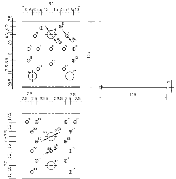
Figure A.6 Dimensions of Angle Bracket A105 without rib
