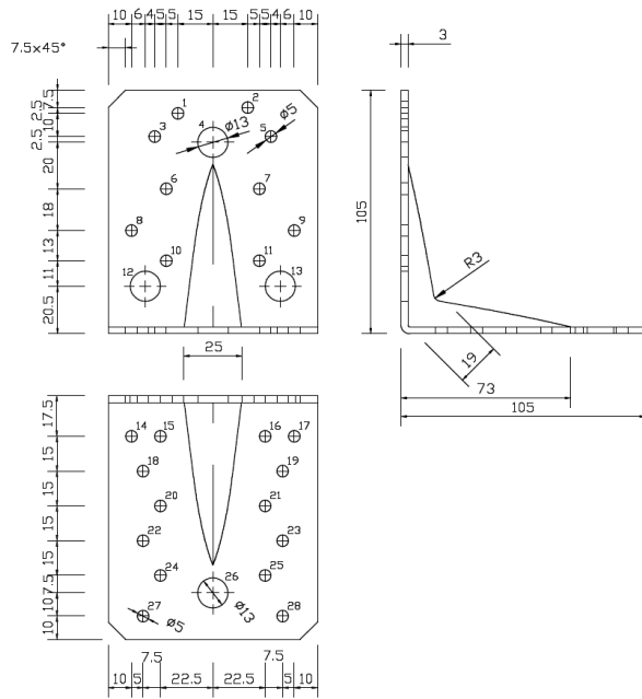
Figure A.5 Dimensions of Angle Bracket A105 with rib
