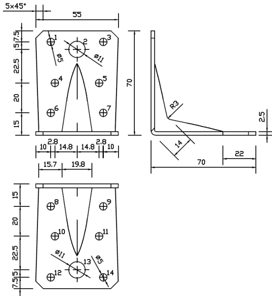
Figure A.1 Dimensions of Angle Bracket A70 with rib
