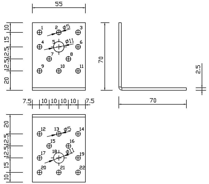
Figure A.2 Dimensions of Angle Bracket A70 without rib
