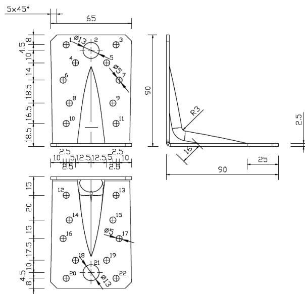
Figure A.3 Dimensions of Angle Bracket A90 with rib
