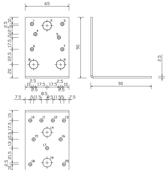
Figure A.4 Dimensions of Angle Bracket A90 without rib
